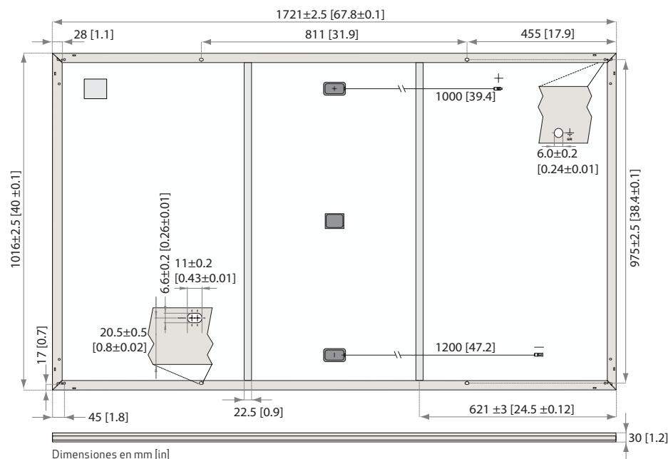
Fig. 19: Dimensiones del panel: REC Alpha Series
