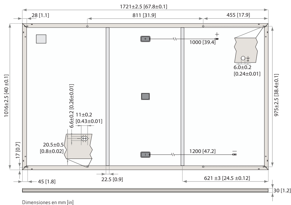
Fig. 20: Dimensiones del panel: REC Alpha Black Series
